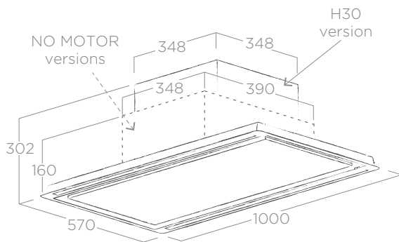
FALSE CEILING CUT: 550X980
